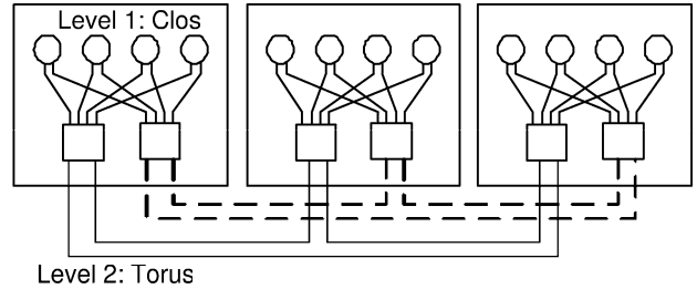
Fig. 2. A hybrid network – a 3-ring of 2-sliced 4-Clos subnetworks
