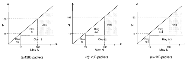
Fig. 7. Latency-optimal topology vs network size for various packet sizes.
