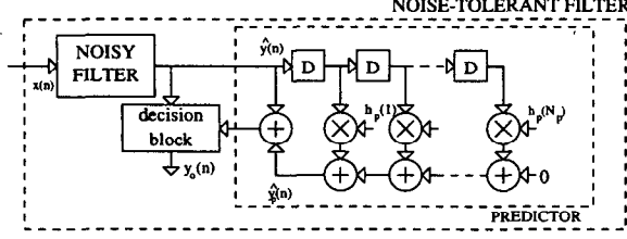
Figure 7: Prediction-based algorithmic noise-tolerance.
