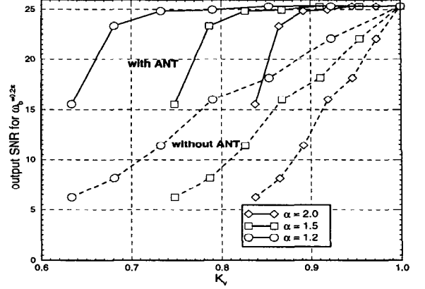
Figure 9: K_v vs. SNR_o for several values of \alpha for the proposed SMA
