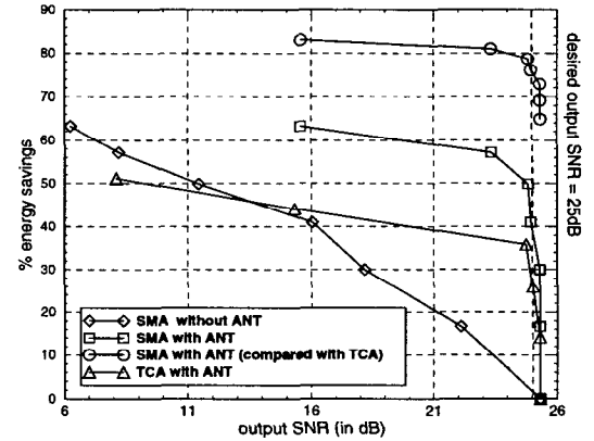
Figure 10: Performance vs. Energy Savings ( \alpha = 1.2 ) with filter bandwidth \omega_b = 0.2\pi for the difference-based ANT scheme.
