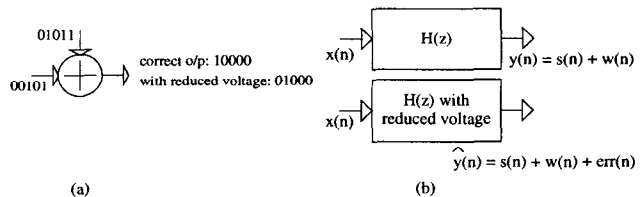
Figure 2: Effect of errors on performance of DSP algorithms
