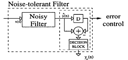
Figure 6: Difference-based ANT scheme for LPF.
